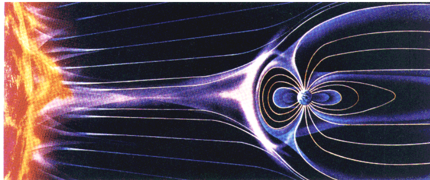
Earth and the Solar Wind
